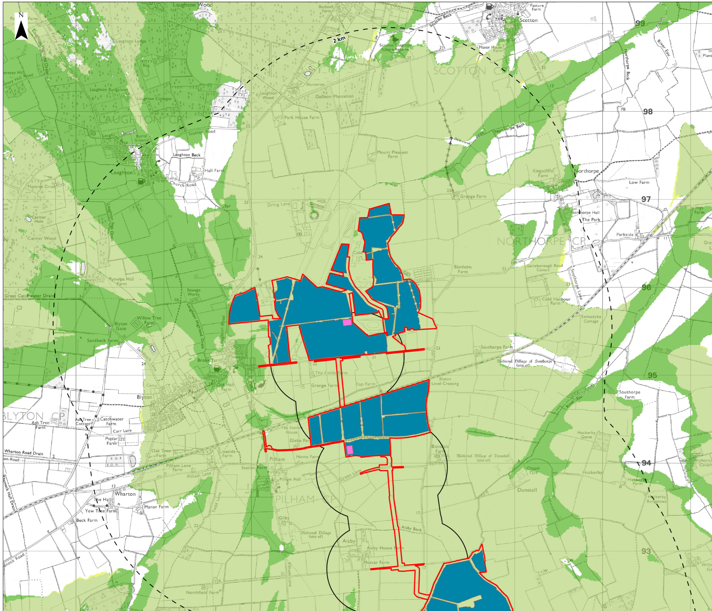
Figure 8.10 Cottam 3 Bare Earth ZTV COTTAM SOLAR PROJECT Landscape and Visual Impact Assessment Environmental Statement (ES)
